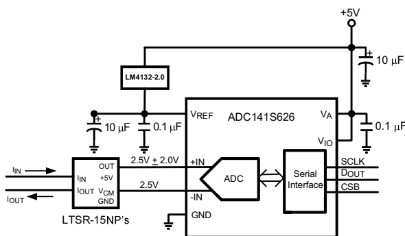
Figure 16. Interfacing the ADC141S626 to a Current Transducer
