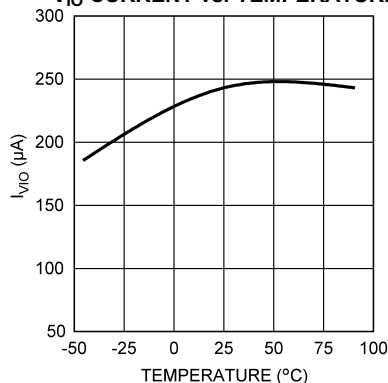
V_{IO} CURRENT vs. TEMPERATURE
