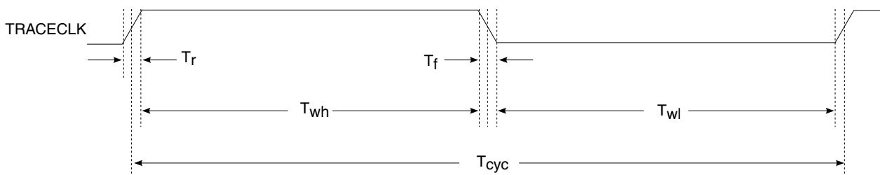
Figure 8. TRACE_CLKOUT specifications
