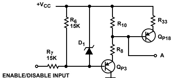
FIGURE 8. SIMPLIFIED SCHEMATIC OF ENABLE/DISABLE FUNCTION
