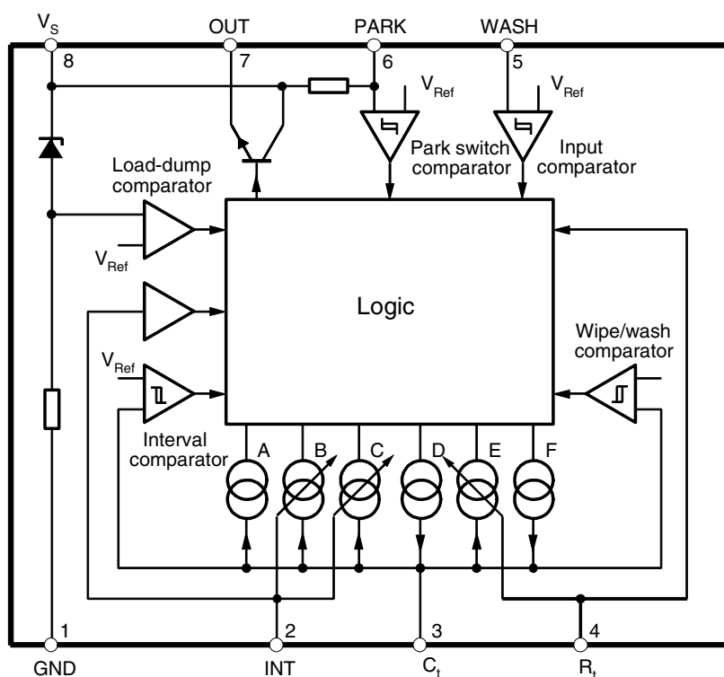
Figure 1. Block Diagram
