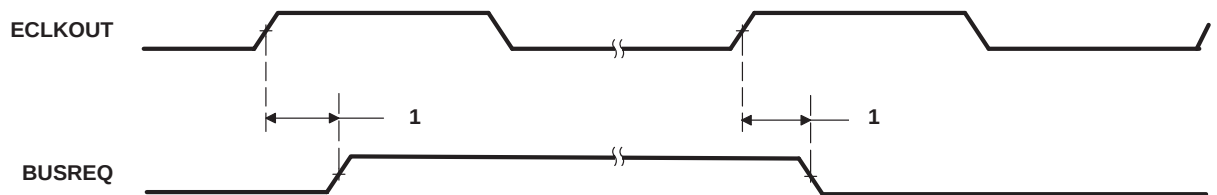
Figure 40. BUSREQ Timing
