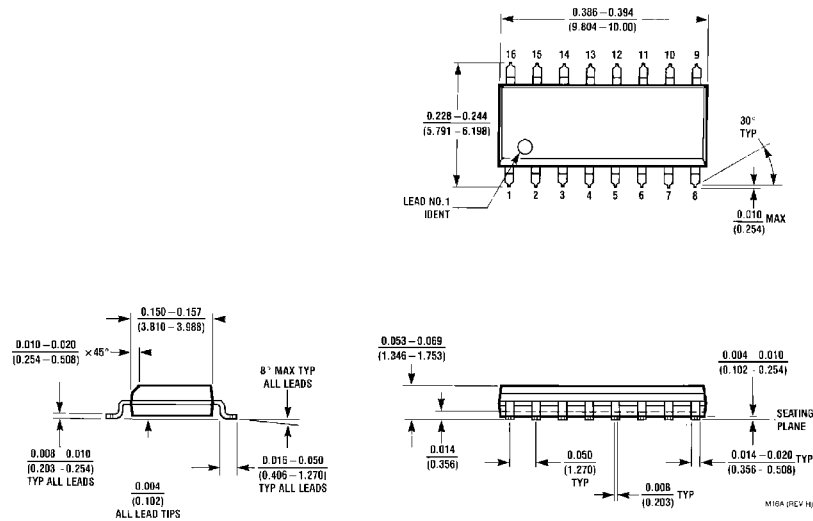
S.O. Package (M) Order Number DM74ALS151M Package Number M16A
