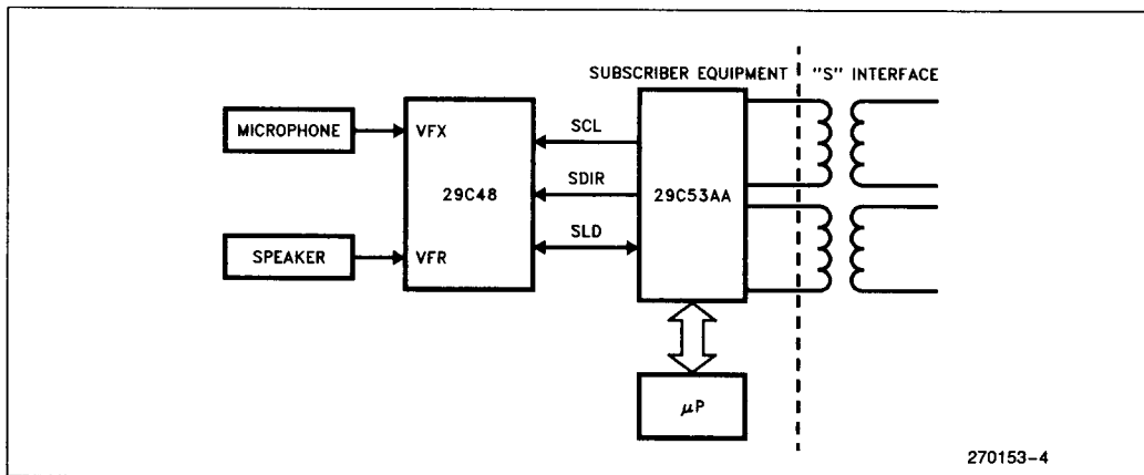
Figure 3. Subscriber Equipment
