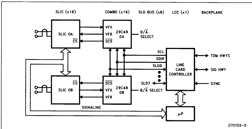
Figure 4a. Analog Line Card with Discrete or Electronic Parallel Control SLICs
