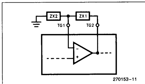
Figure 8a. Transmit Frequency Compensation
