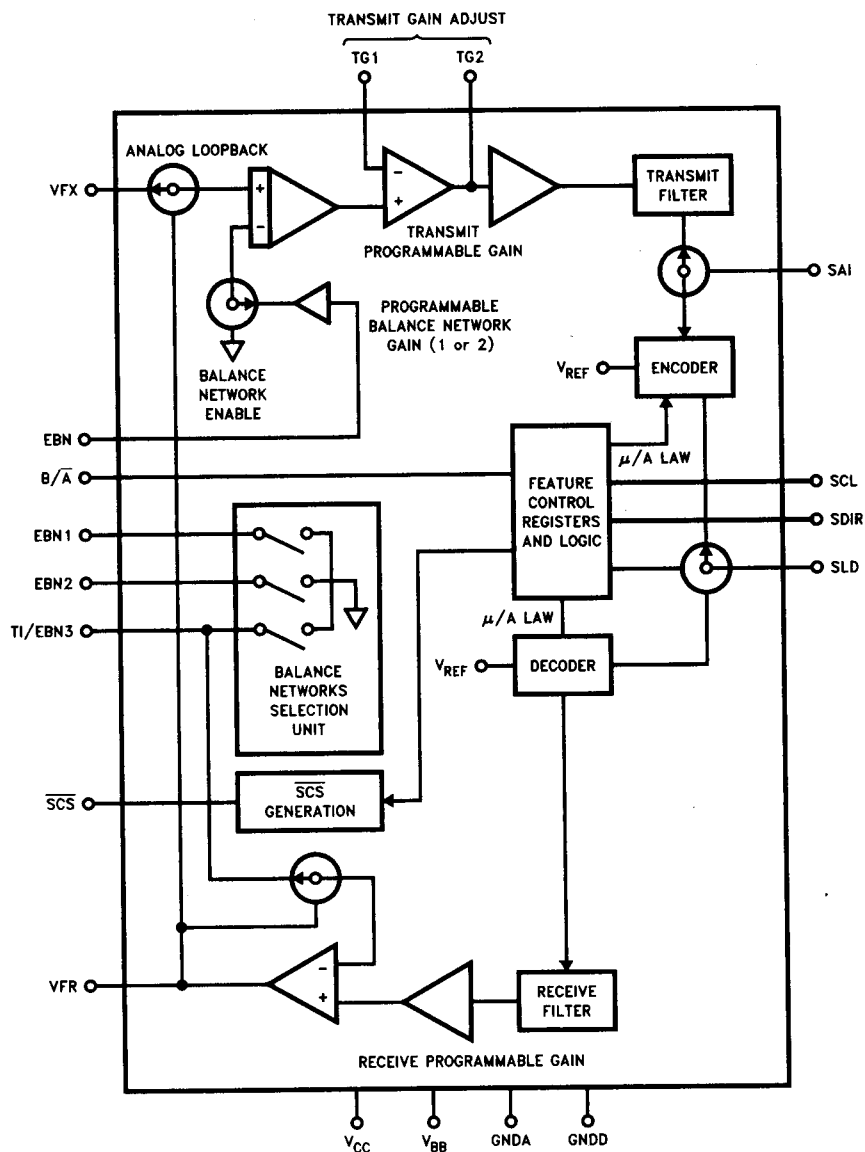
Figure 2. Block Diagram
