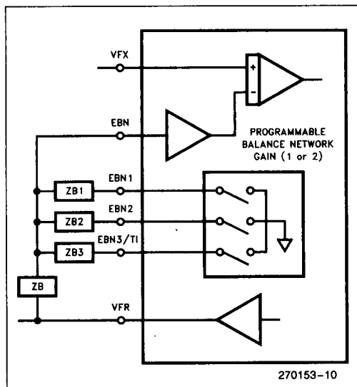
Figure 7. Balance Networks
