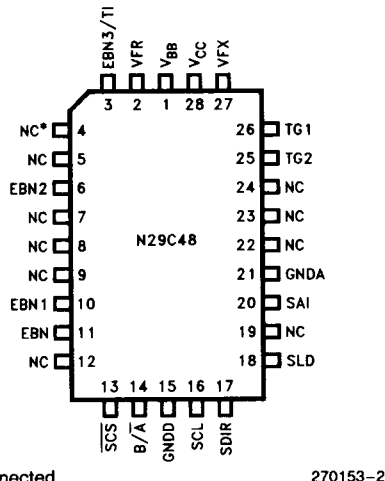
Plastic Leaded Chip Carrier
