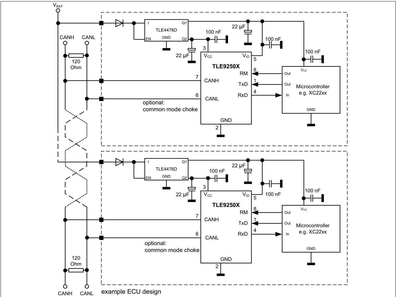
Figure 15 Application circuit
