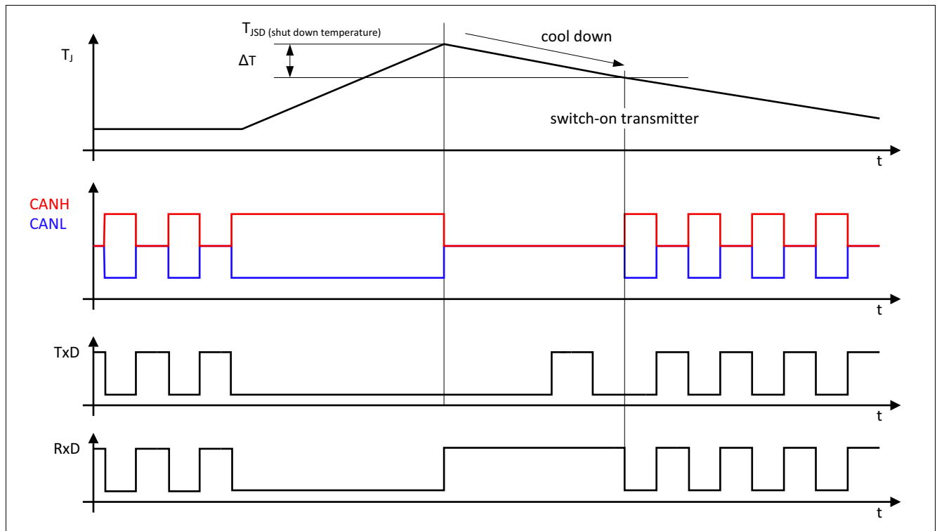
Figure 11 Overtemperature protection
