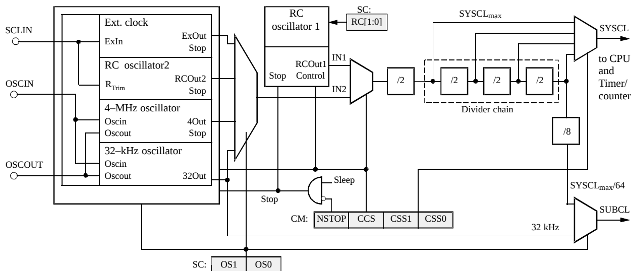
Figure 11. Clock module
