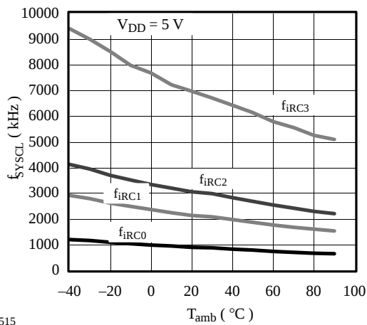
Figure 57. f_{SYSCL} = f(T_{amb})
