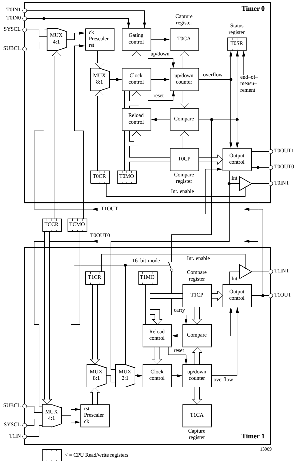
Figure 28. Timer/counter module
