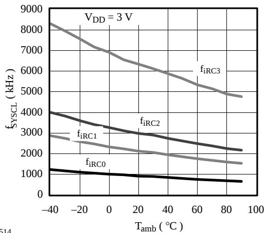
Figure 56. f_{SYSCL} = f(T_{amb})
