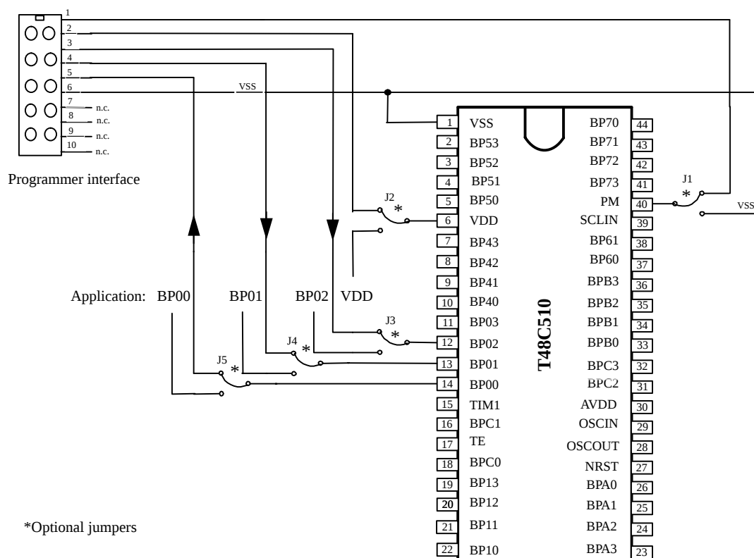
Figure 47. In-system programming
