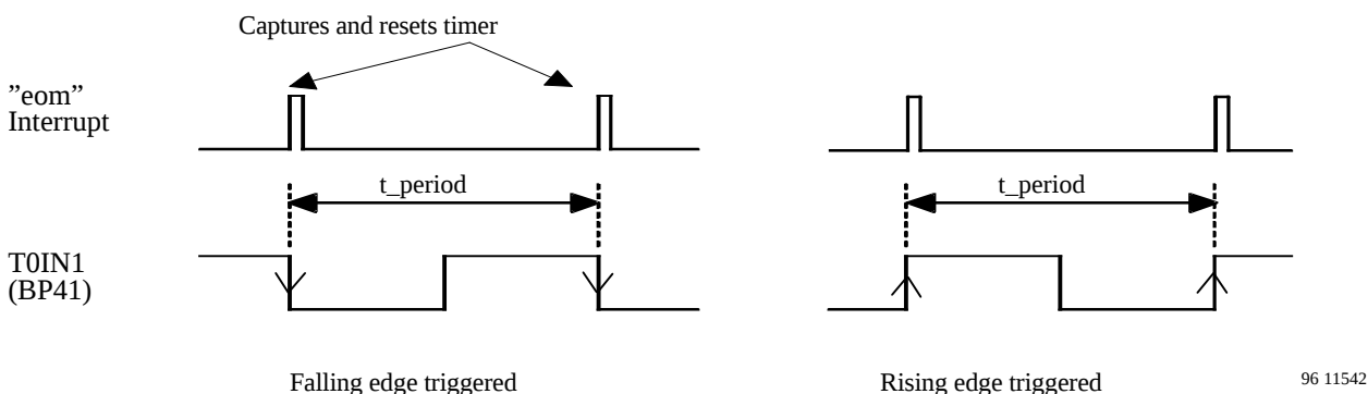
Figure 37. Period measurement
