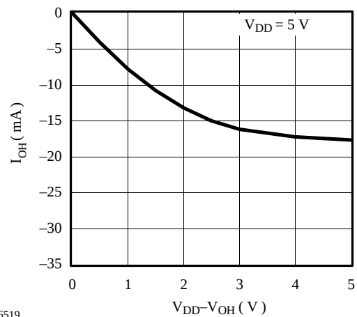
Figure 61. Typical high output driver
