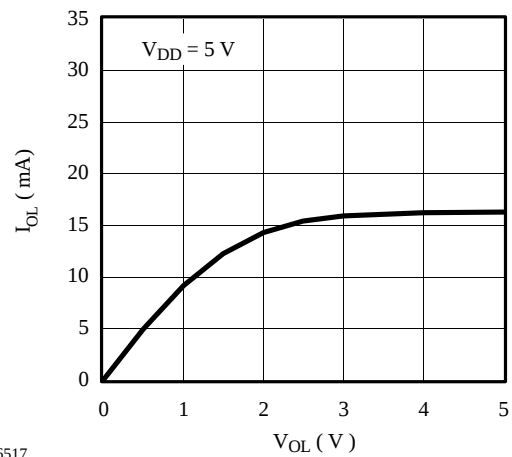
Figure 60. Typical low output driver
