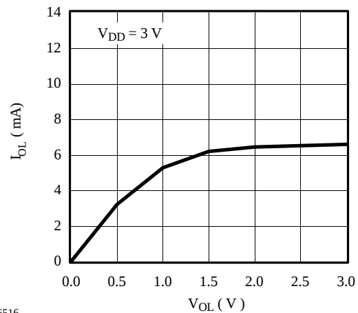
Figure 59. Typical low output driver
