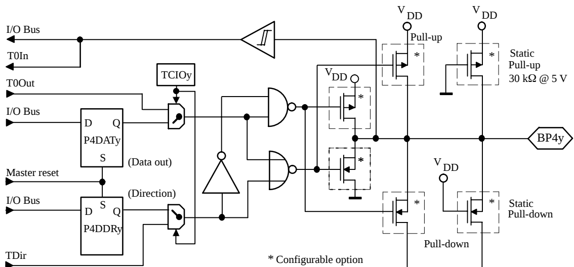
Figure 24. Bidirectional Port 4
