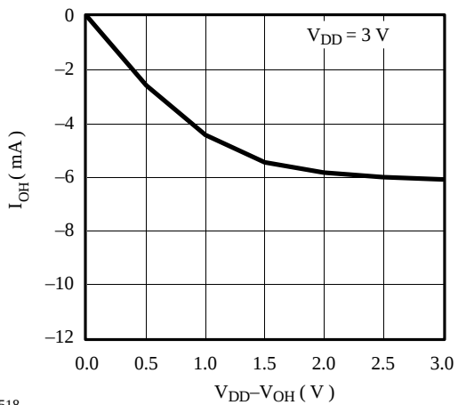
Figure 58. Typical high output driver
