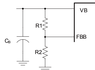
Figure 6. Release Feedback Circuit
