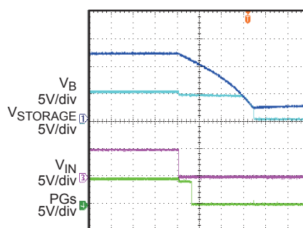
V_{STORAGE} Release
