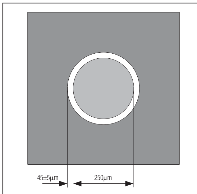
Figure 15. PCB Footprint Recommendation Diagram
