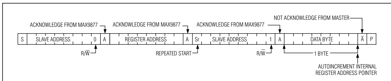
Figure 11. Reading One Indexed Byte of Data from the MAX9877
