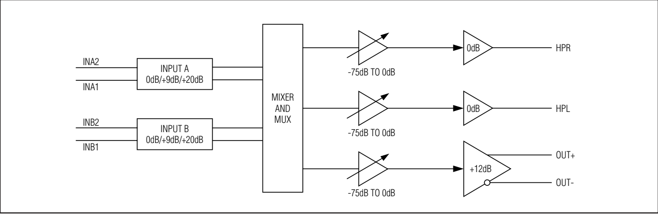
Figure 1. Signal Path
