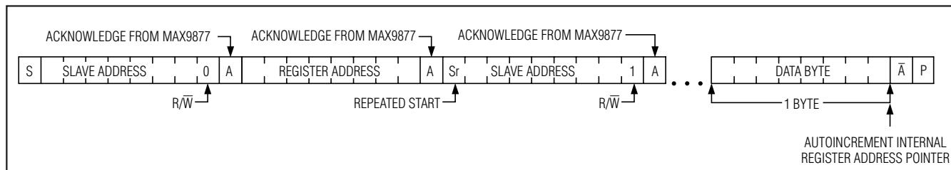
Figure 12. Reading n-Bytes of Indexed Data from the MAX9877
