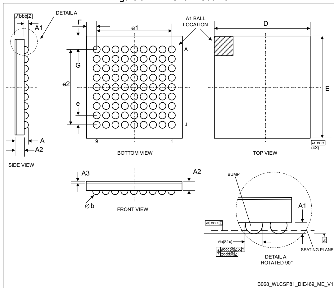
Figure 54. WLCSP81 - Outline
