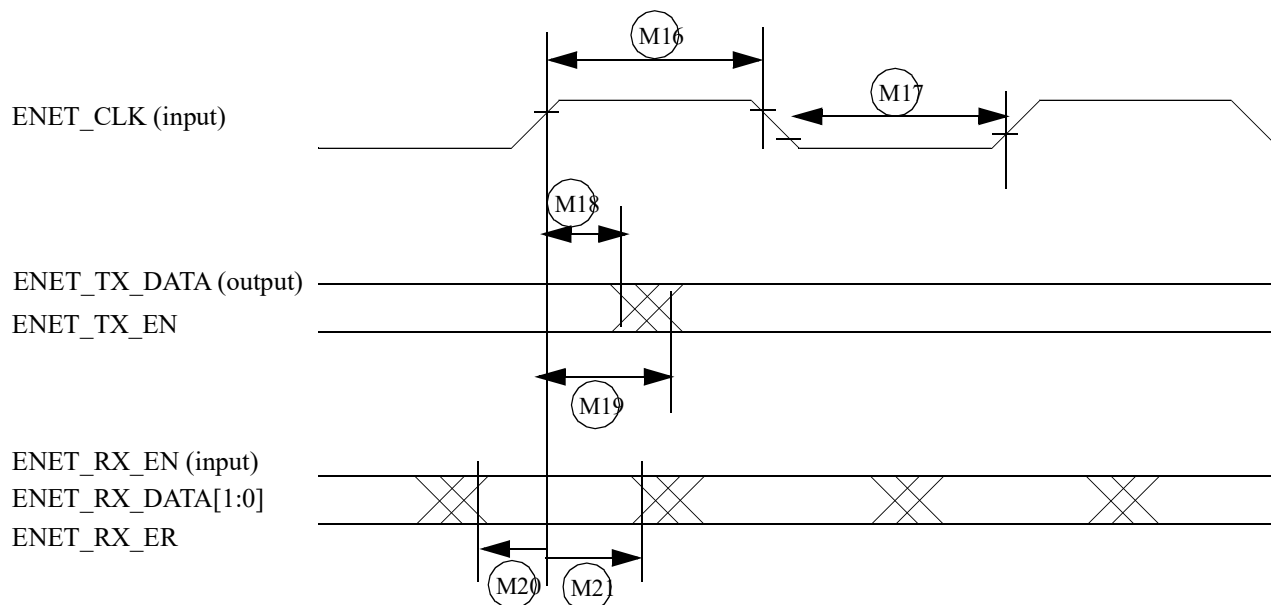
Figure 47. RII mode signal timing diagram
