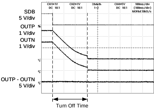
Figure 24. Turn Off Waveform
