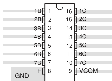
Figure 11-1. Package Layout
