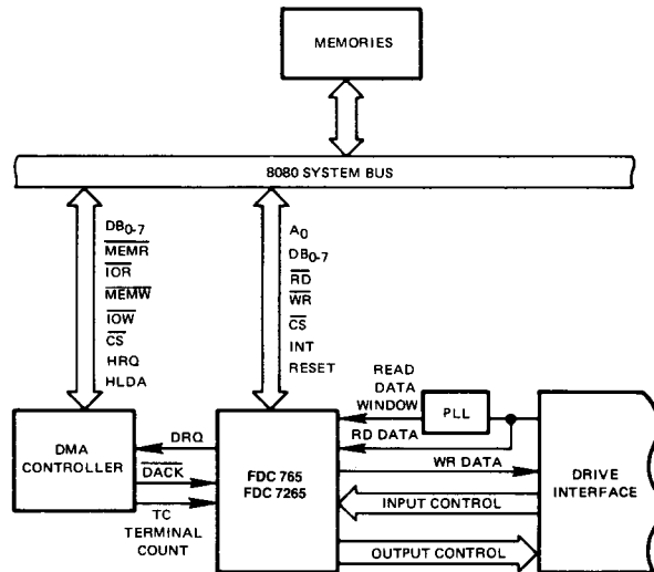
SYSTEM CONFIGURATION
