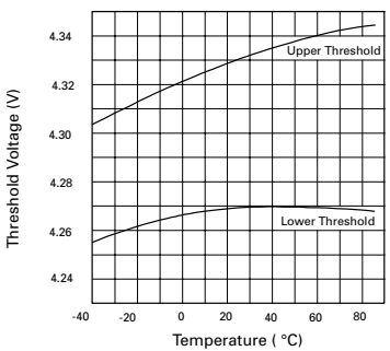
Threshold Voltage vs. Temperature
