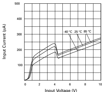
Input Current vs. Input Voltage
