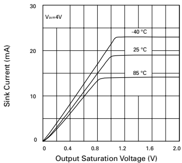
Output Saturation Voltage vs. Sink Current
