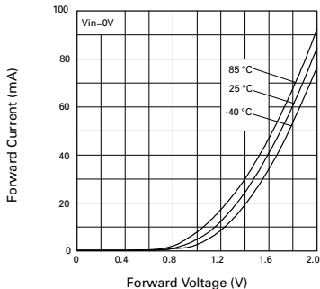
Clamp Diode Forward Current vs. Voltage
