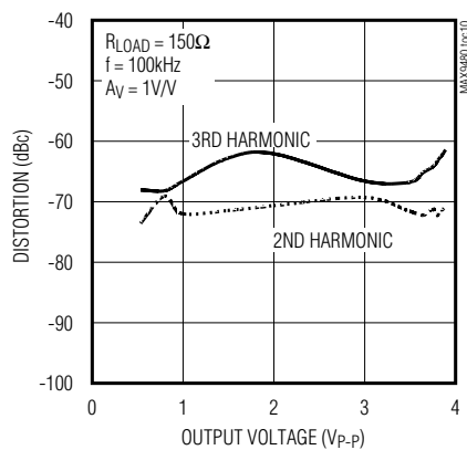
RECEIVER AMPLIFIER HARMONIC DISTORTION vs. OUTPUT AMPLITUDE
