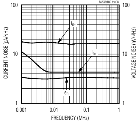
RECEIVER INPUT NOISE vs. FREQUENCY
