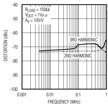
RECEIVER AMPLIFIER HARMONIC DISTORTION vs. FREQUENCY
