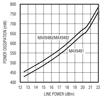
POWER DISSIPATION vs. LINE POWER
