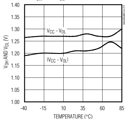
V OH AND V OL vs. TEMPERATURE
