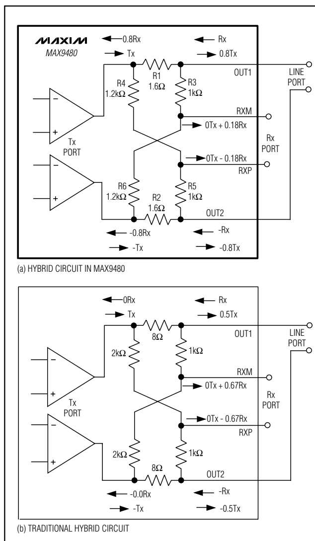
Figure 6. Hybrid Circuit in the MAX9480
