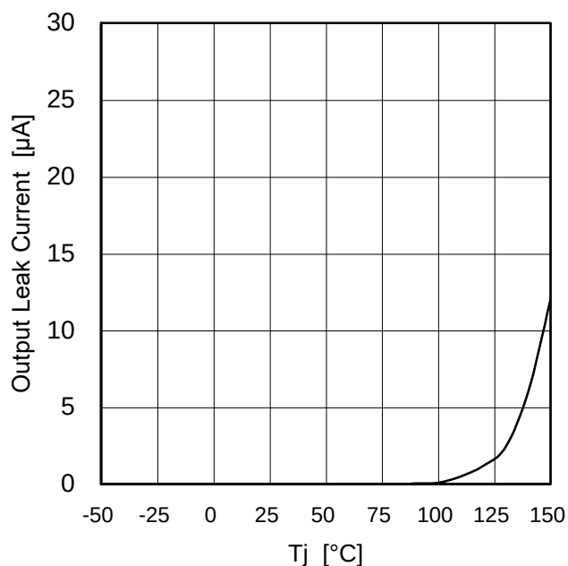
Figure 15. Output Leak Current [Temperature Characteristic] (V IN =0V)
