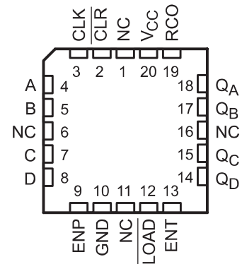
SN54HC163 . . . FK PACKAGE (TOP VIEW)
