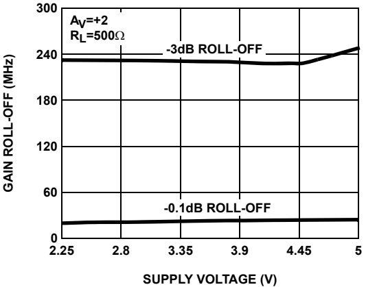
FIGURE 4. GAIN ROLL-OFF vs FREQUENCY
