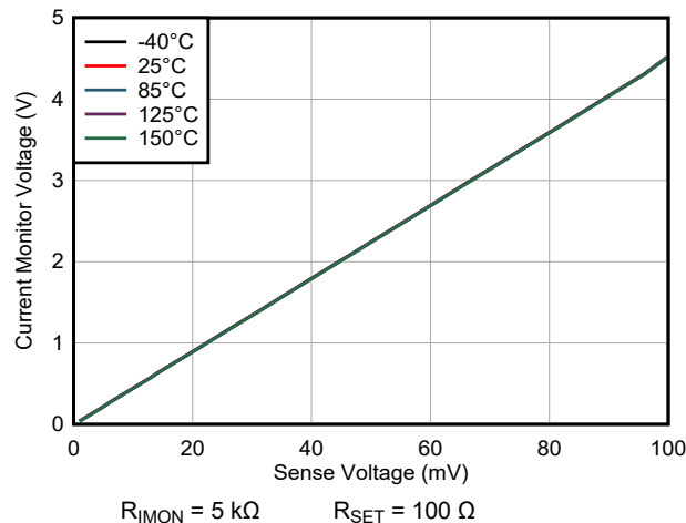
Figure 7-9. Current Monitor Voltage ( V_{(IMON)} ) vs Sense Voltage ( V_{(SNS)} )
