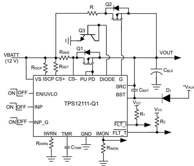
Figure 9-5. TPS12111-Q1 Application Circuit with external supply to BST
