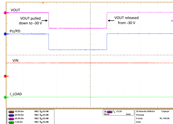
Figure 9-16. Output Short to -30 V Response with VIN = 12 V and INP = LOW
