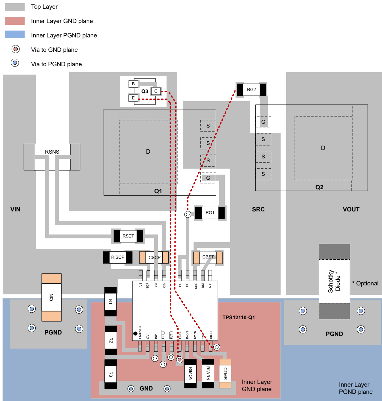
Figure 10-17. Typical PCB Layout Example for TPS12110-Q1 with B2B MOSFETs
