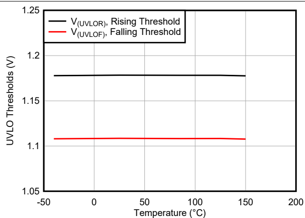
Figure 7-14. Input Supply UVLO Thresholds vs Temperature
