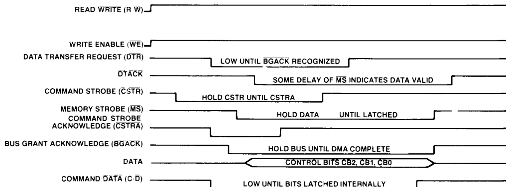
FIGURE 1: BUS CONTROLLER TIMING SEQUENCE
