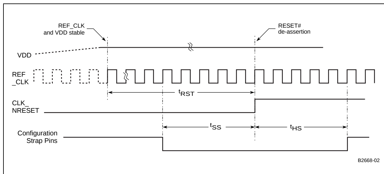
Figure 27. Reset Timing
