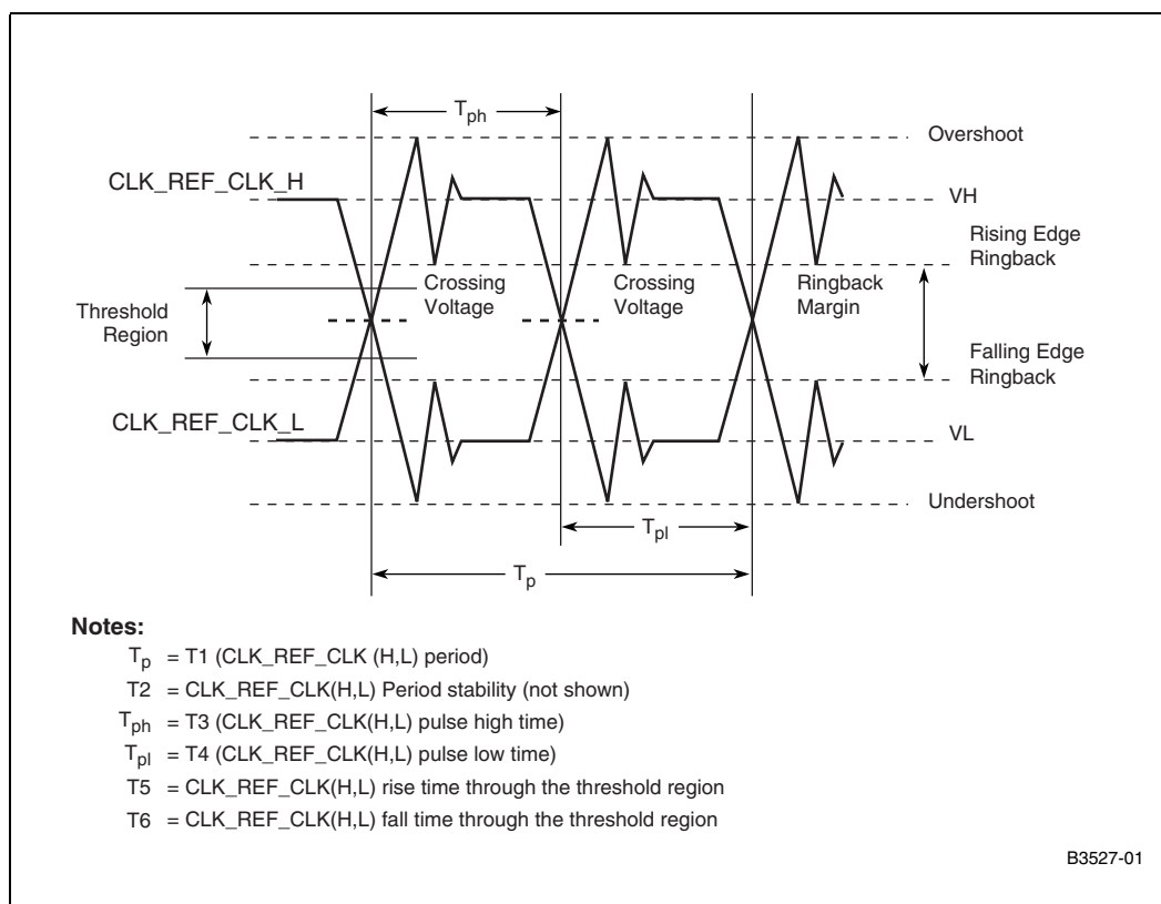
Figure 11. REF_CLK Timing
