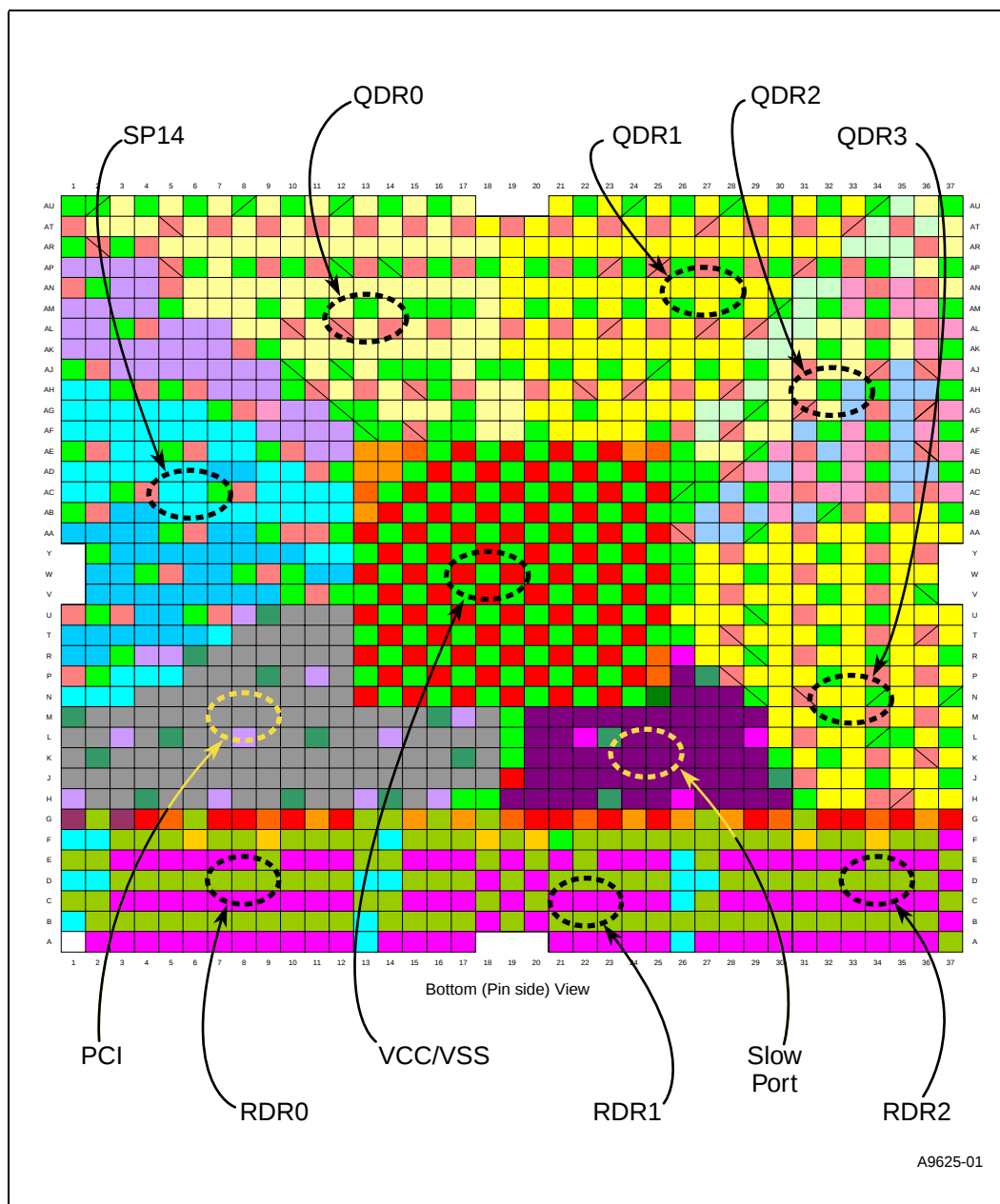
Figure 9. Pinout Diagram
