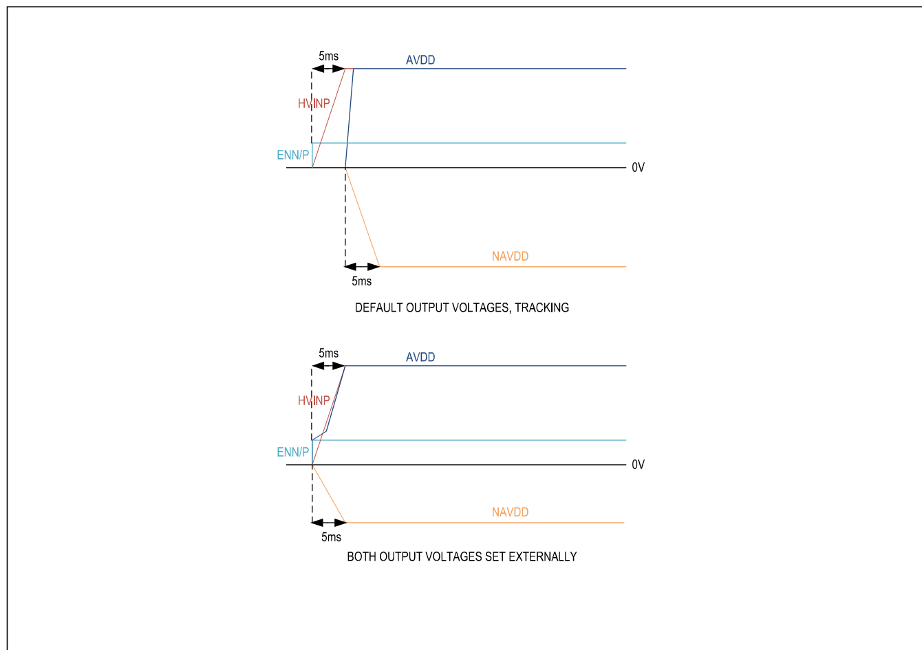
Figure 1. Start-Up Waveforms
