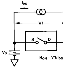
Test Circuit 1
