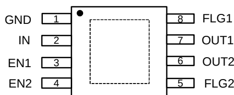
MSOP-8EP
