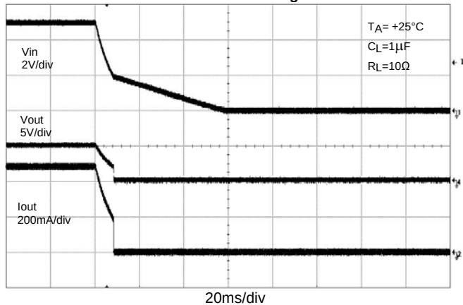
UVLO Decreasing
