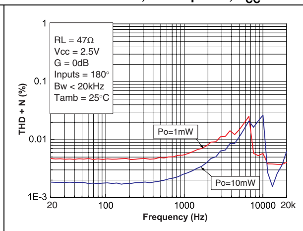
Figure 51. THD+N vs. frequency RL = 47\ \Omega , out-of-phase, V_{CC} = 2.5\ V
