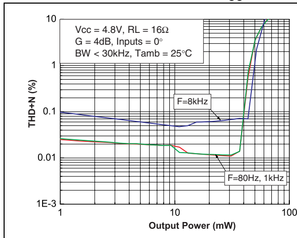
Figure 24. THD+N vs. output power RL = 16\ \Omega , in-phase, V_{CC} = 4.8\ V
