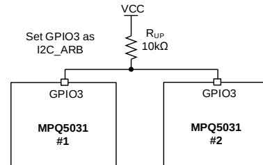
Figure 14: I 2 C Arbitration Connection
