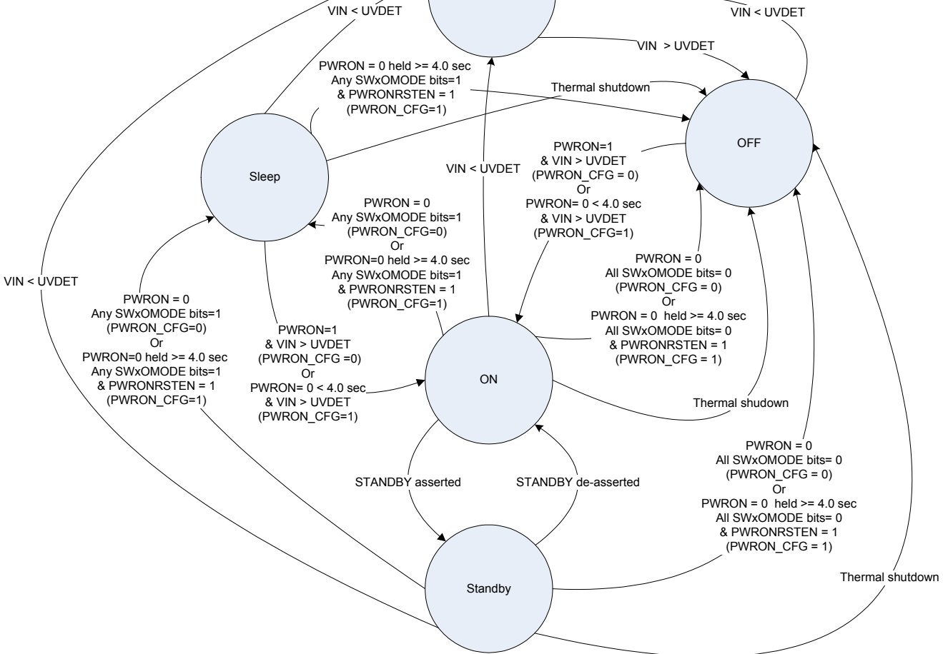
Figure 8. State Diagram
