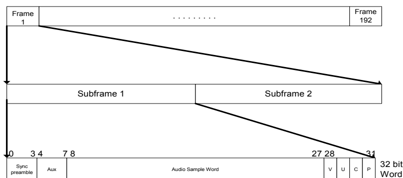
Figure 33 S/PDIF Format
