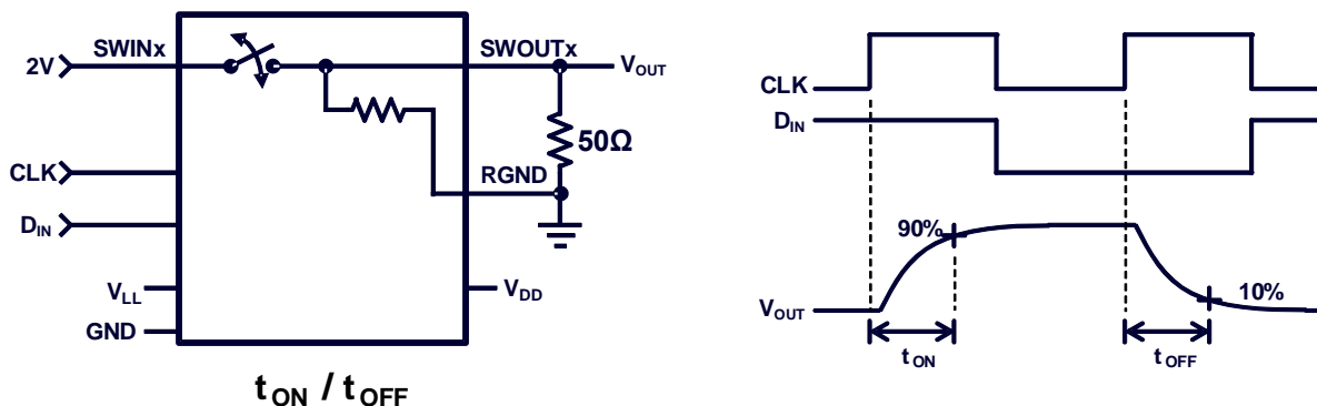
Figure 5: Test Circuit 4
