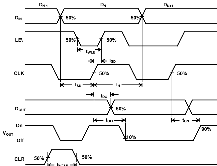
Figure 1: Timing Diagram
