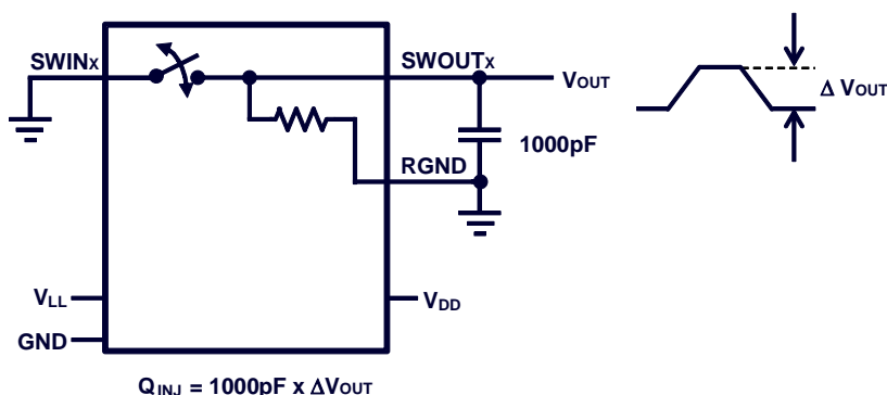
Figure 9: Test Circuit 8
