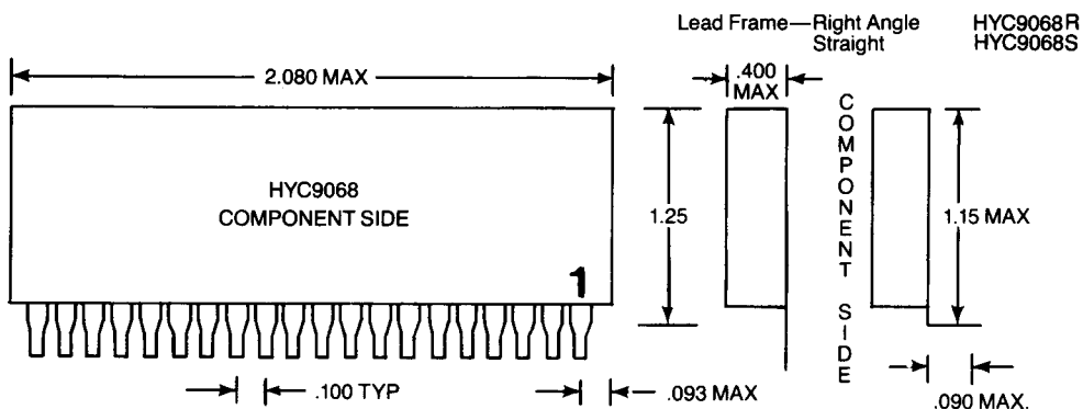
FIGURE 3—MECHANICAL SPECIFICATION
