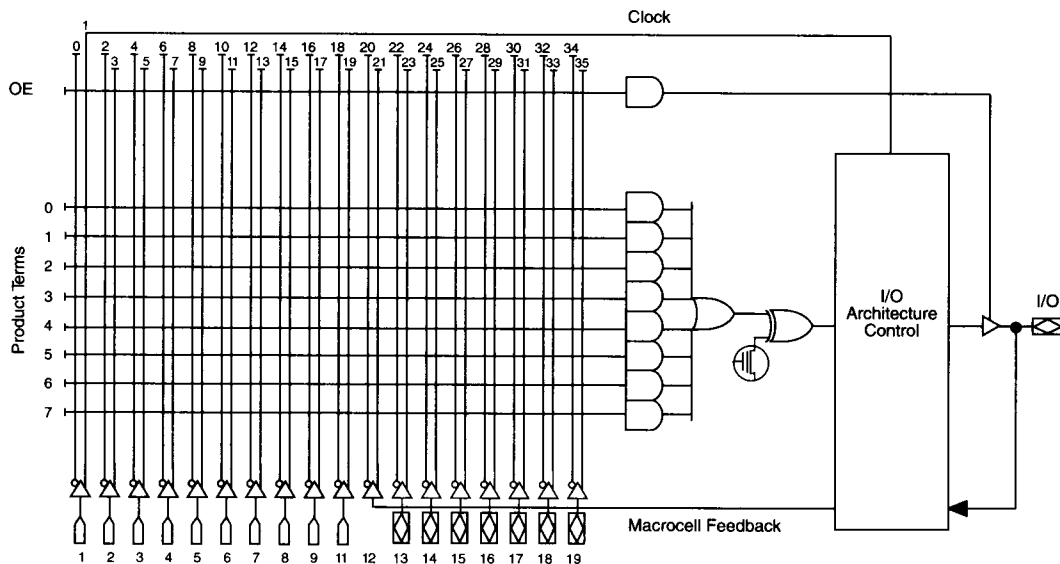
Figure 3. EP330 Macrocell
