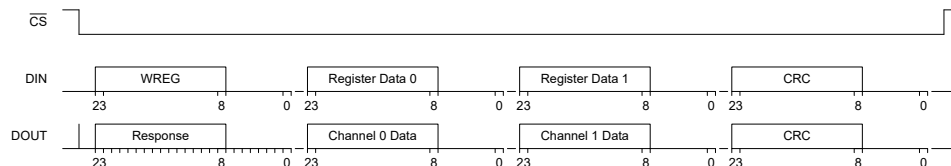
Figure 8-15. SPI Frame using 24-bit, zero-padded Word Size
