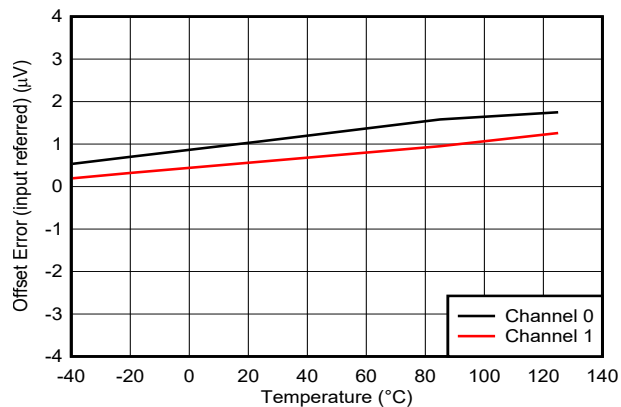
Figure 6-5. Offset Error vs Temperature
