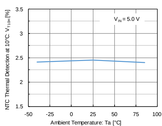
(37) Thermistor Detection Hysteresis at 10°C vs. Ambient Temperature
