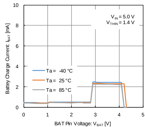
(9) Battery Charge Current vs. BAT Pin Voltage ( R_{ISET} = 59 \text{ k}\Omega , Cold Operation)
