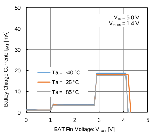
(13) Battery Charge Current vs. BAT Pin Voltage ( R_{\text{SET}} = 5.9 \text{ k}\Omega , Cold Operation)
