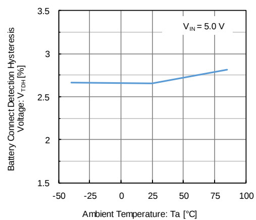
(33) Battery Connect Detection Hysteresis Voltage vs. Ambient Temperature
