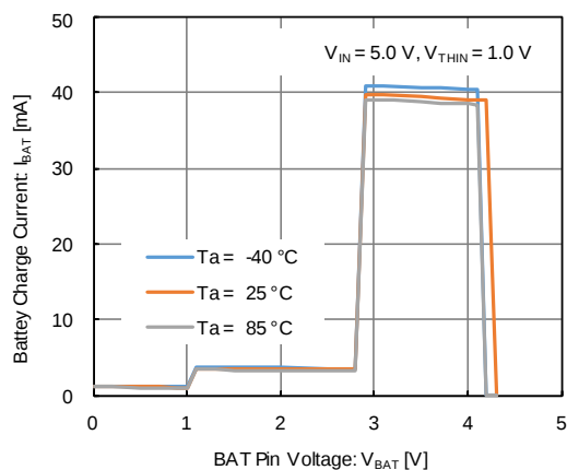
(12) Battery Charge Current vs. BAT Pin Voltage ( R_{\text{SET}} = 5.9 \text{ k}\Omega , Normal Operation)
