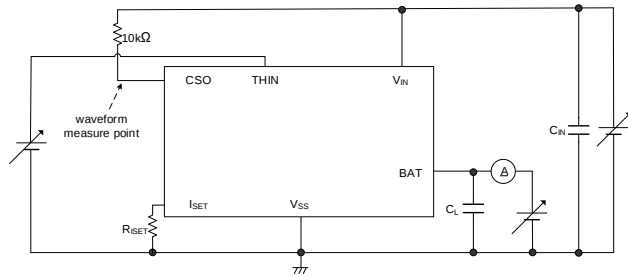
2) Test Circuit ②
