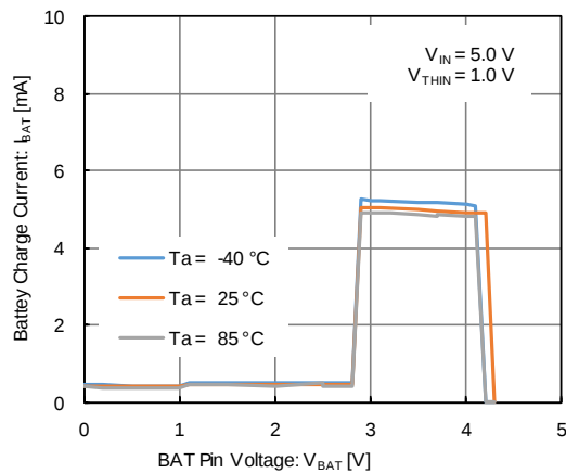
(8) Battery Charge Current vs. BAT Pin Voltage ( R_{ISET} = 59 \text{ k}\Omega , Normal Operation)
