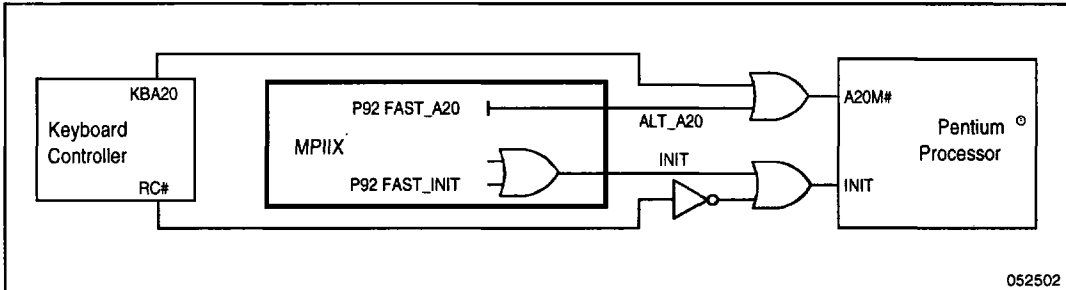
Figure 2. Fast A20Gate and INIT Connections
