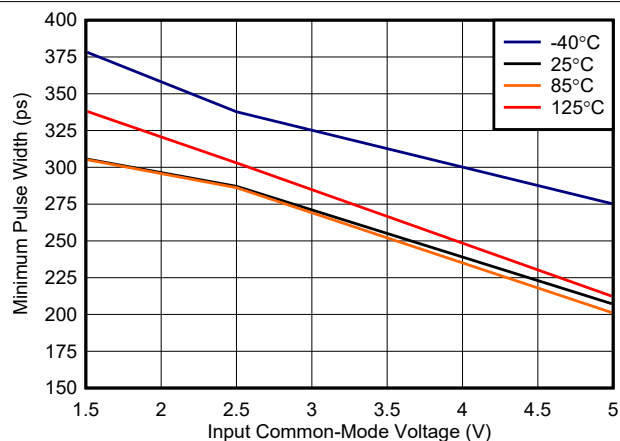
Figure 6-22. Minimum Pulse Width vs. Common-Mode, 5 V
