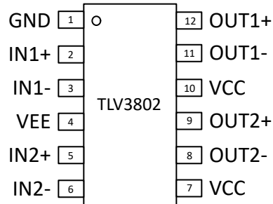
Figure 5-3. WF-DFN Package 12-Pin DSS Top View
