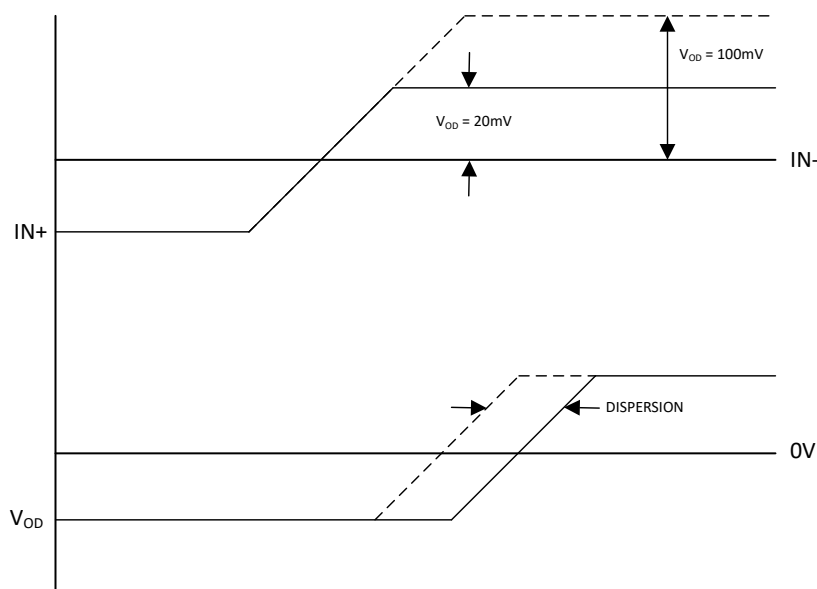
Figure 6-2. Overdrive Dispersion
