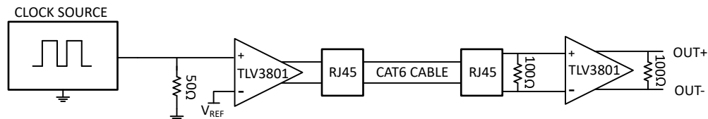
Figure 8-5. LVDS Clock Transceiver
