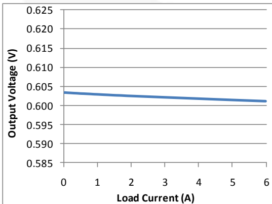
Figure 10. Load Regulation
