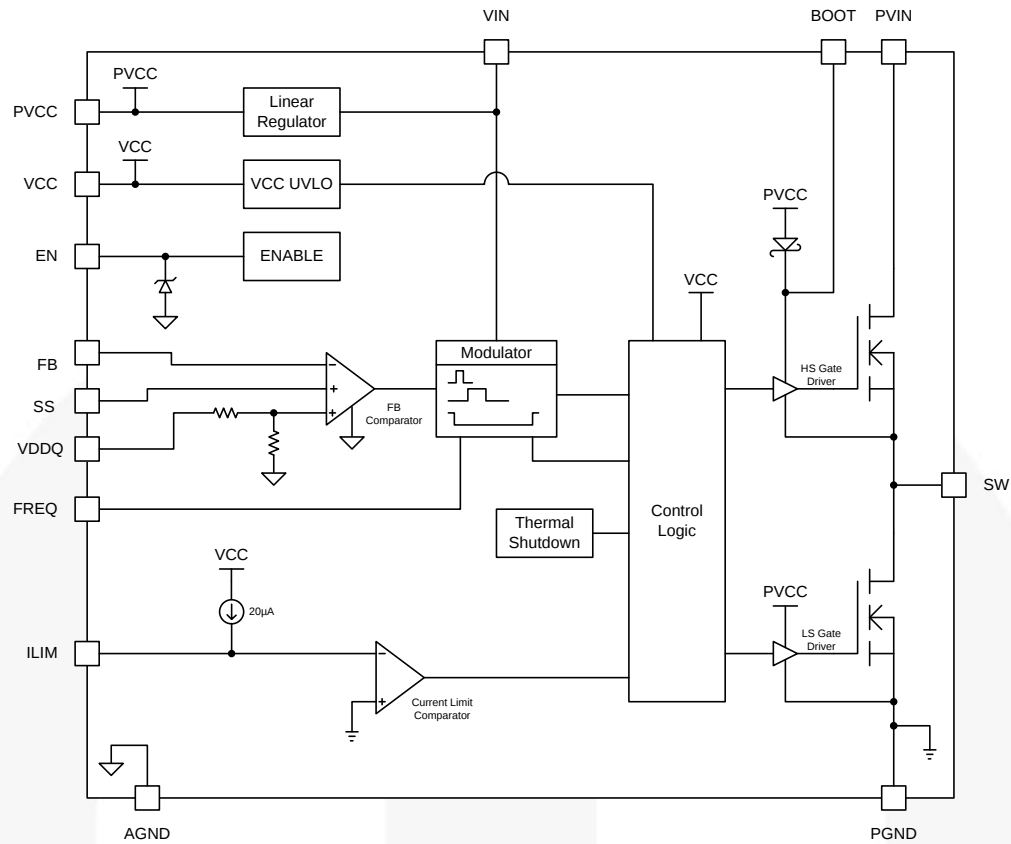
Figure 3. Block Diagram
