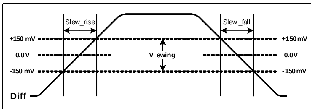
Figure 5. Differential Measurements
