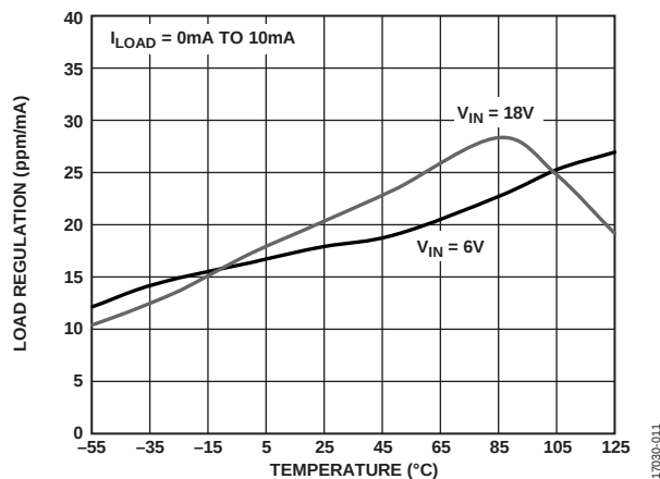
Figure 7. Load Regulation vs. Temperature for Various Input Voltages
