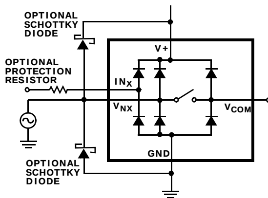
FIGURE 9. OVERVOLTAGE PROTECTION
