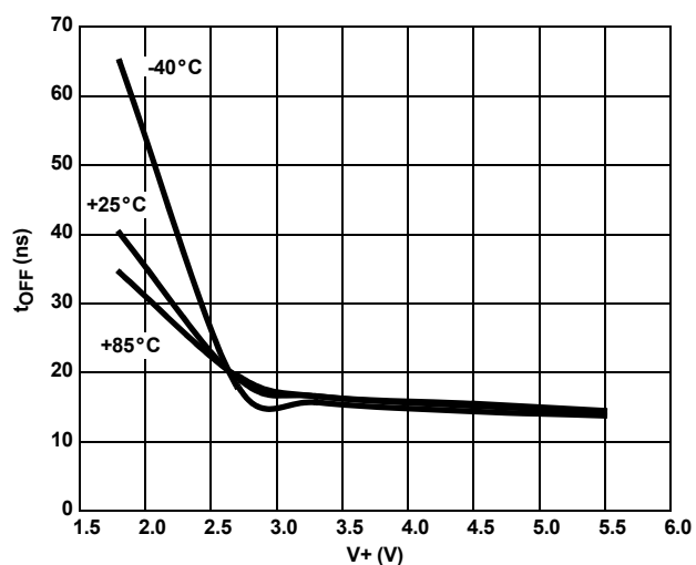
FIGURE 15. TURN-OFF TIME vs SUPPLY VOLTAGE
