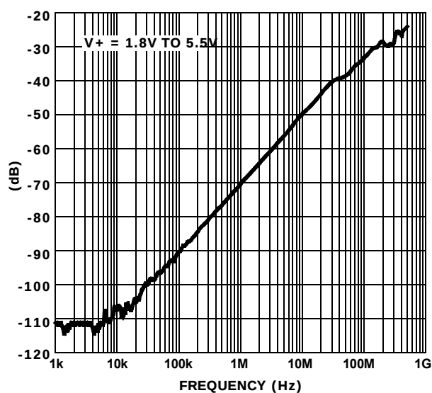
FIGURE 18. OFF-ISOLATION
