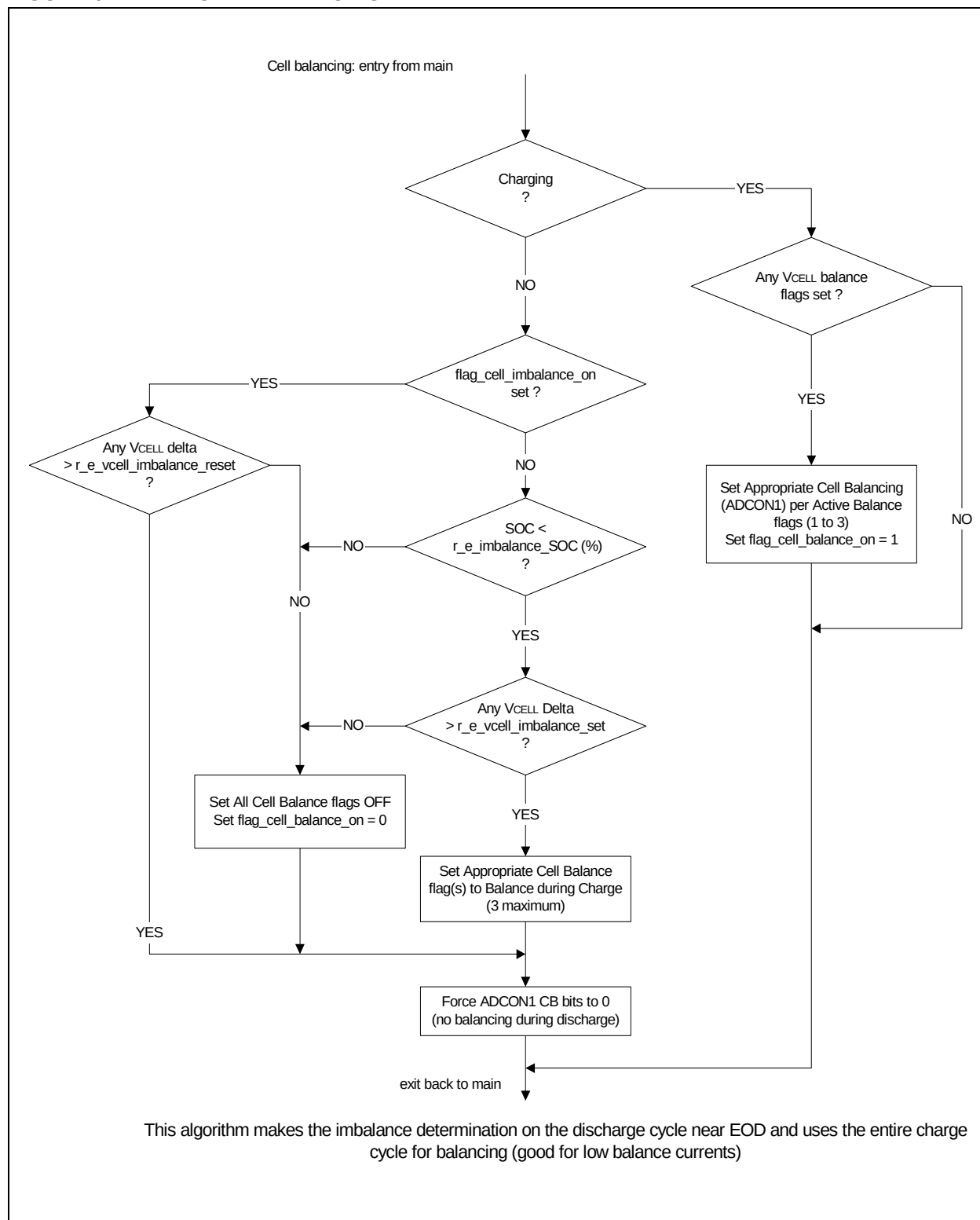
FIGURE 6-1: CELL BALANCING
