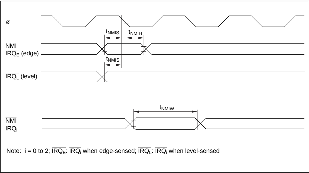
Figure 16-7 Interrupt Input Timing
