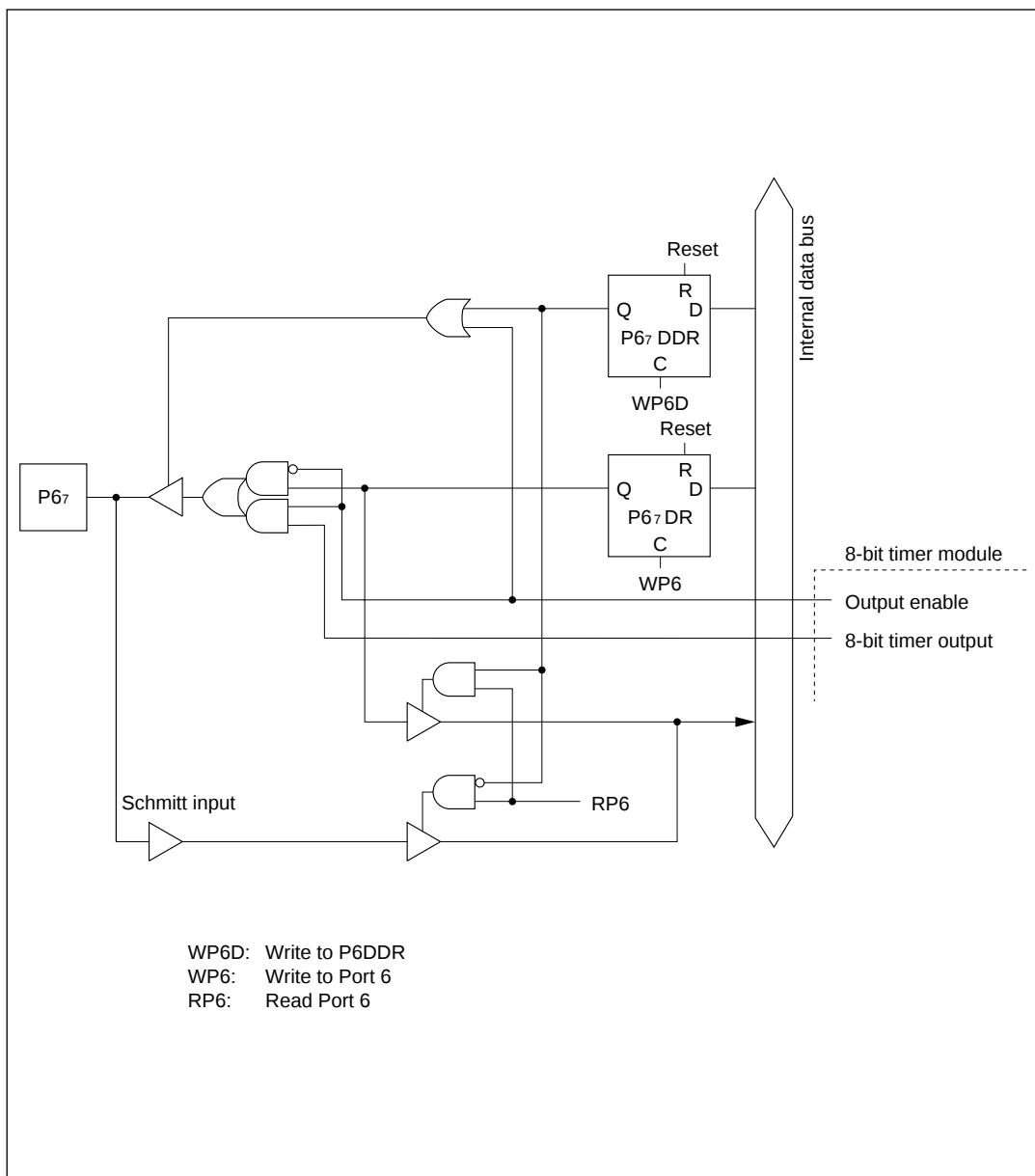
Figure C-6 (g) Port 6 Block Diagram (Pin P67)
