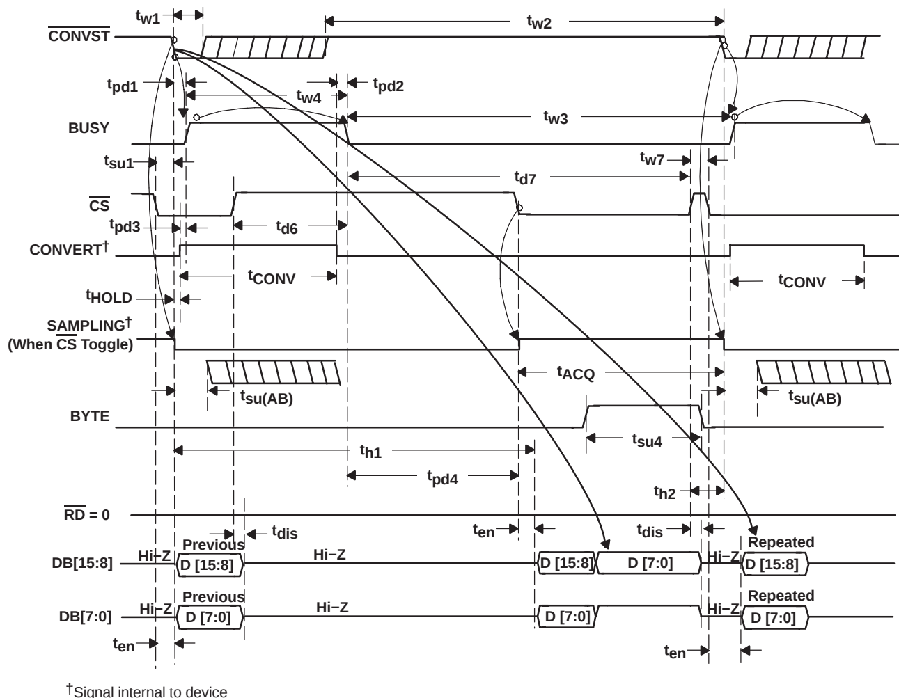
Figure 2. Timing for Conversion and Acquisition Cycles With \overline{\text{CS}} Toggling, \overline{\text{RD}} Tied to \text{BDGND}
