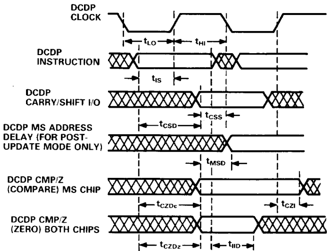
Figure 2. Supplemental Parameters for Double-Chip/Double-Precision Operation
