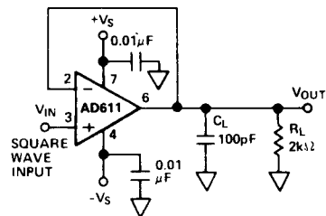
Figure 13c. Unity Gain Follower
