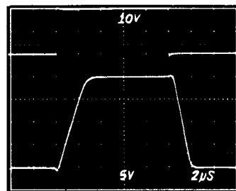
Figure 15b. Large Signal Response
