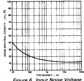
Figure 6. Input Noise Voltage Spectral Density
