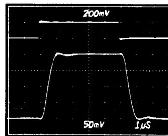
Figure 15c. Small Signal Response
