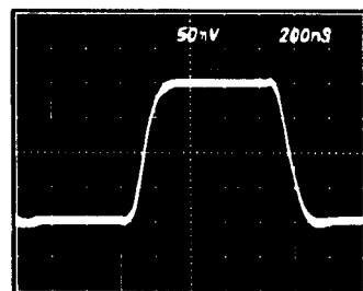
Figure 14c. Unity Gain Inverter Pulse Response (Small Signal)
