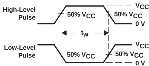
VOLTAGE WAVEFORMS PULSE DURATIONS
