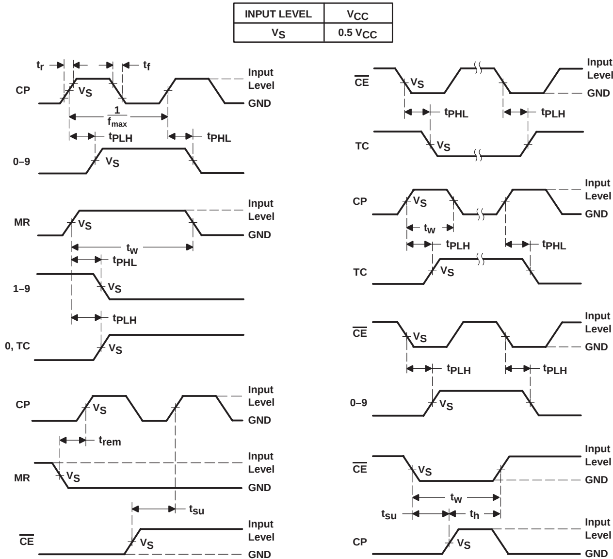
Figure 2. Voltage Waveforms
