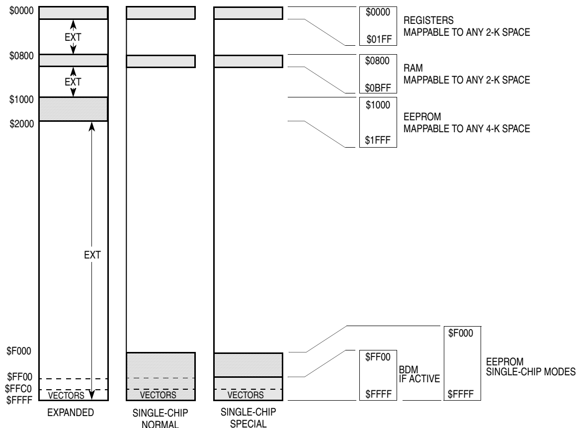
Figure 5-6. Memory Map
