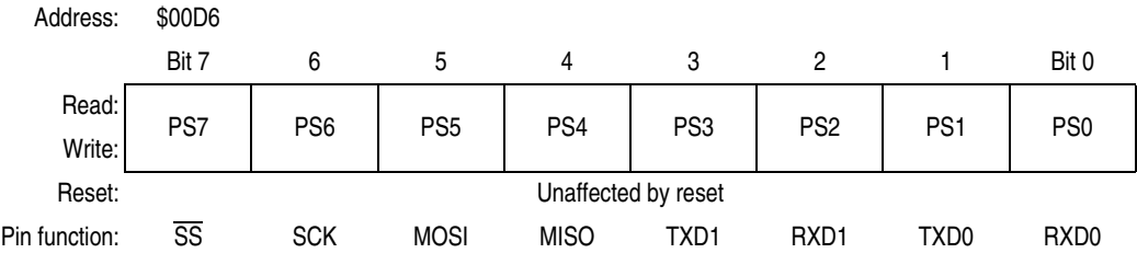
Figure 13-3. Port S Data Register (PORTS)
