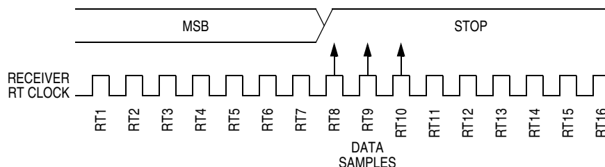
Figure 14-13. Slow Data
