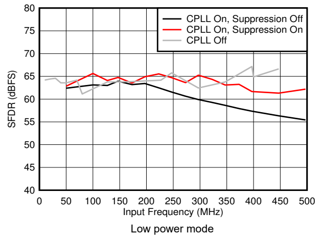
Figure 7-44. SFDR vs F_{IN} and C-PLL modes
