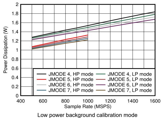
Figure 7-90. Dual Channel, Power Dissipation vs F_S and JMODE 4 - 7
