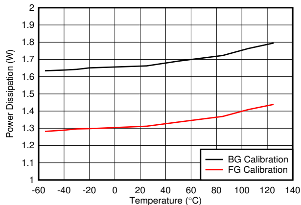
Figure 7-121. Quad Channel, Power Dissipation vs Temperature
