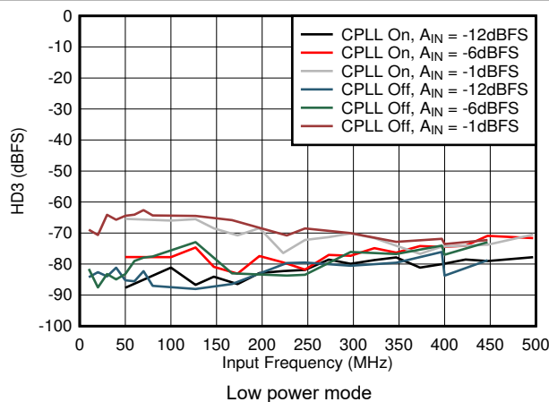
Figure 7-59. HD3 vs A_{IN} and C-PLL
