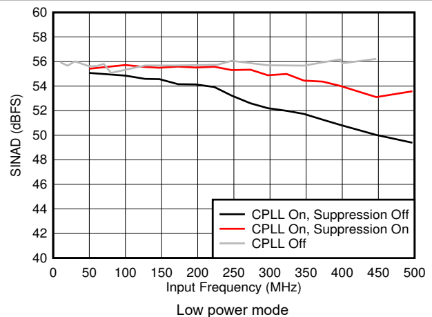
Figure 7-46. SINAD vs F_{IN} and C-PLL modes
