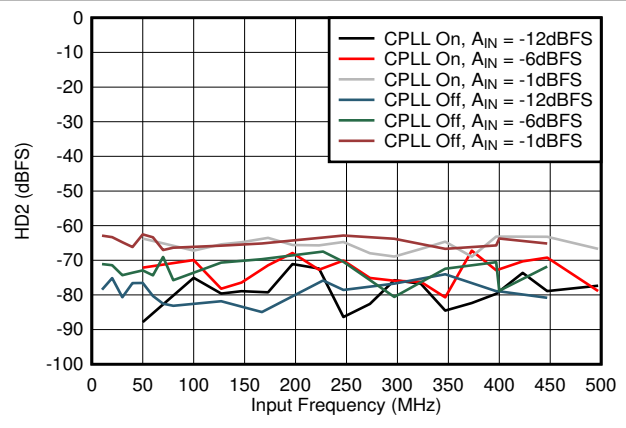
Figure 7-58. HD2 vs A_{IN} and C-PLL
