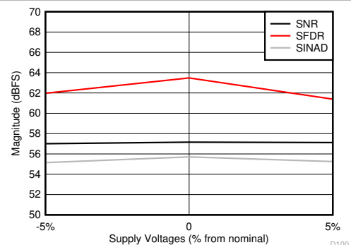
All supplies changed together, high power mode Figure 7-60. SNR, SFDR and SINAD vs Supply Voltage
