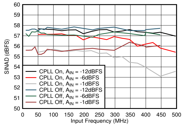
Figure 7-56. SINAD vs A_{IN} and C-PLL
